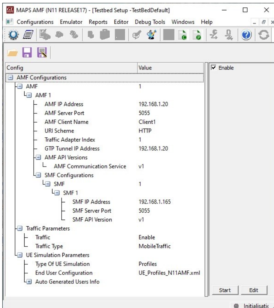
Figure: Testbed Setup
