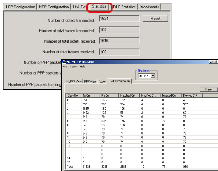
Figure: Statistics and Tx Rx Verification
