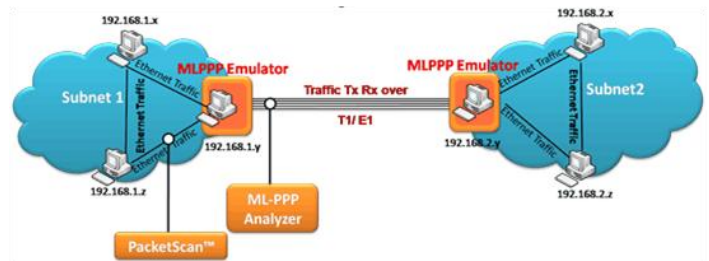
Figure: MLPPP Emulator as a Bridge
