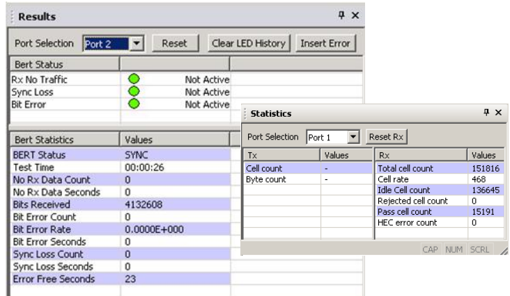
Figure: BERT Results and Statistics
