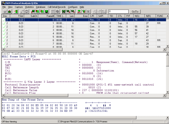
Figure: Summary, Detail, & Hex dump Views
