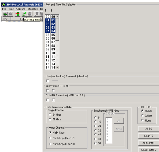
Figure: Stream / Interface Selection
